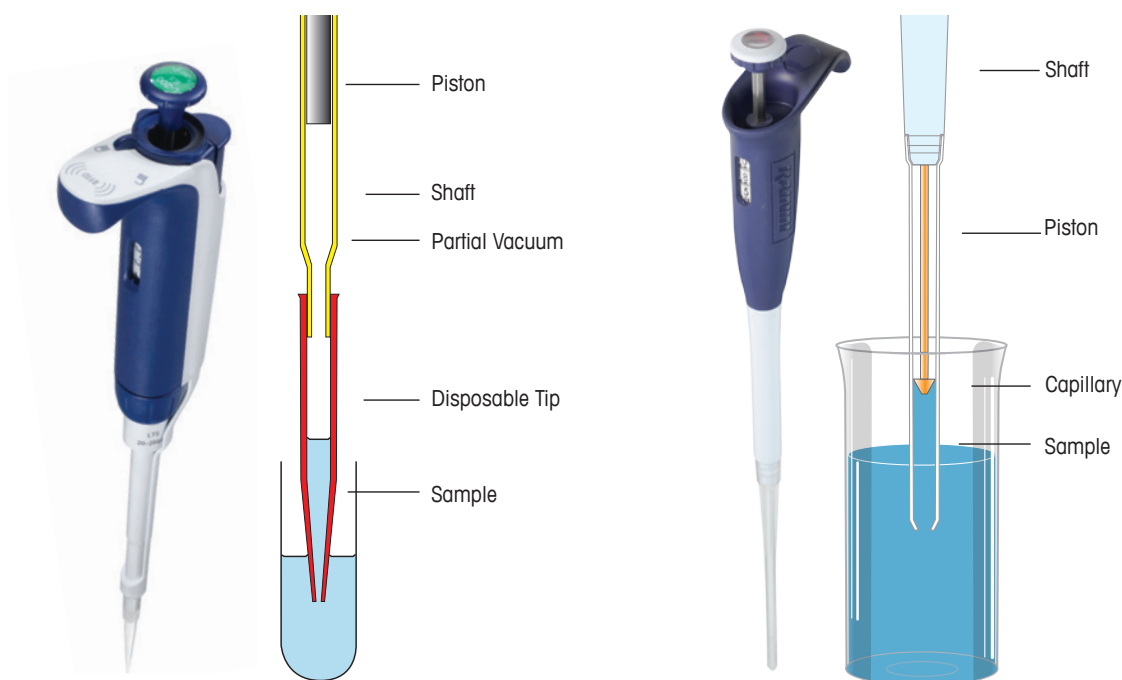
Figure 1: Air and positive displacement pipettes.
